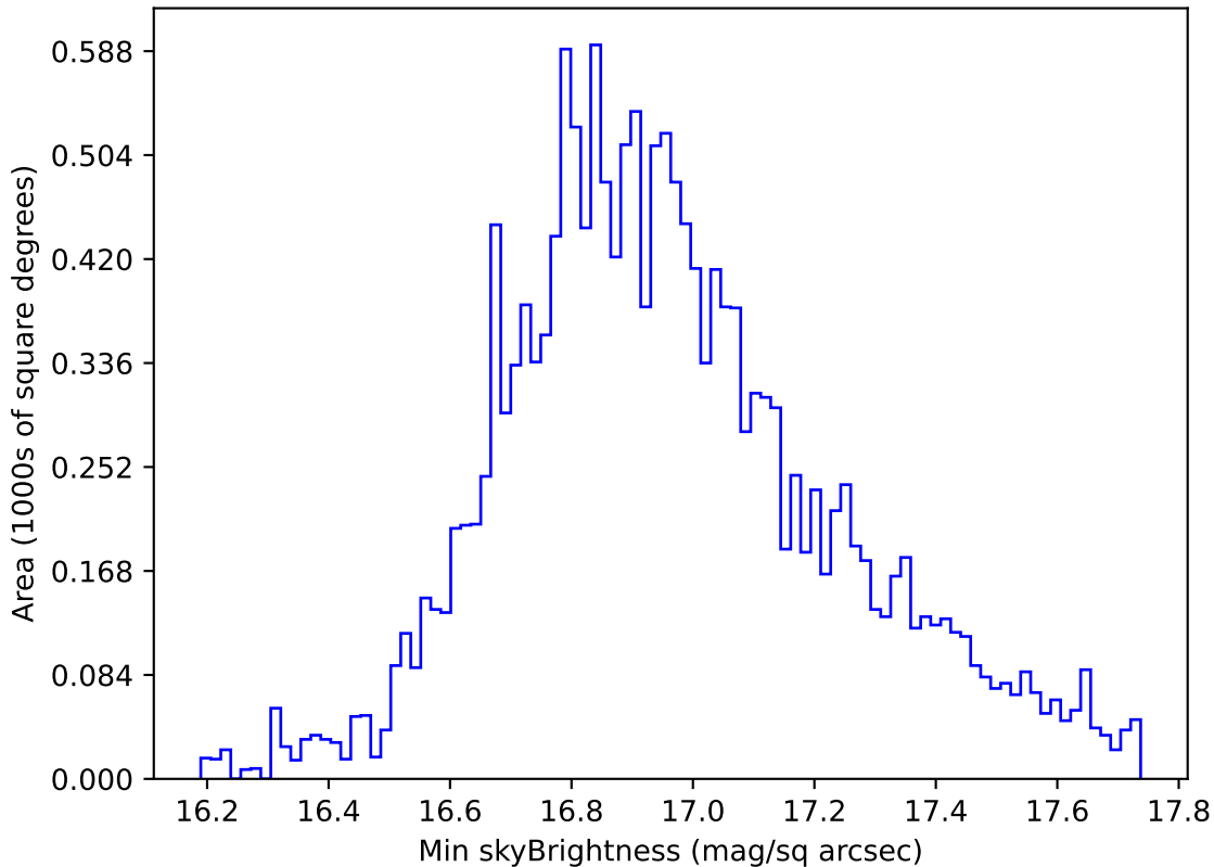
ddf_acor_sf15_lsf40_lsr20_v3.4_10yrs WFD all bands: Min skyBrightness
