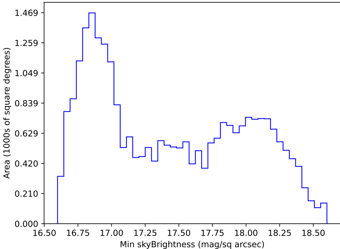
ddf_acor_sf15_lsf40_lsr20_v3.4_10yrs All sky z band: Min skyBrightness
