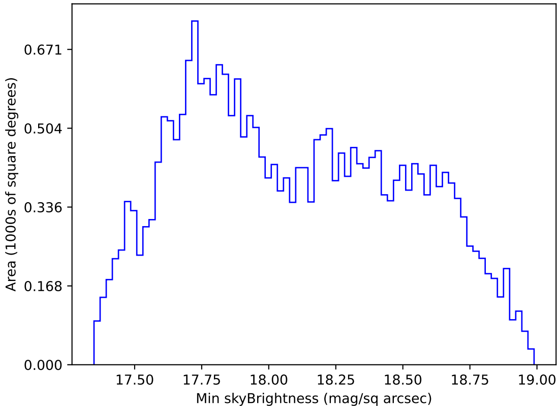
ddf_acor_sf15_ls40_lsr20_v3.4_10yrs All sky i band: Min skyBrightness
