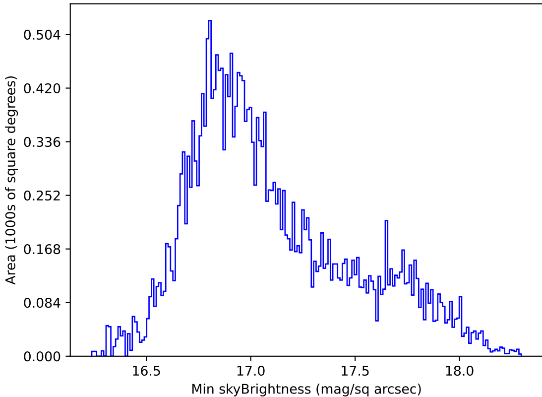
ddf_acor_sf15_lsf40_lsr20_v3.4_10yrs All sky all bands: Min skyBrightness
