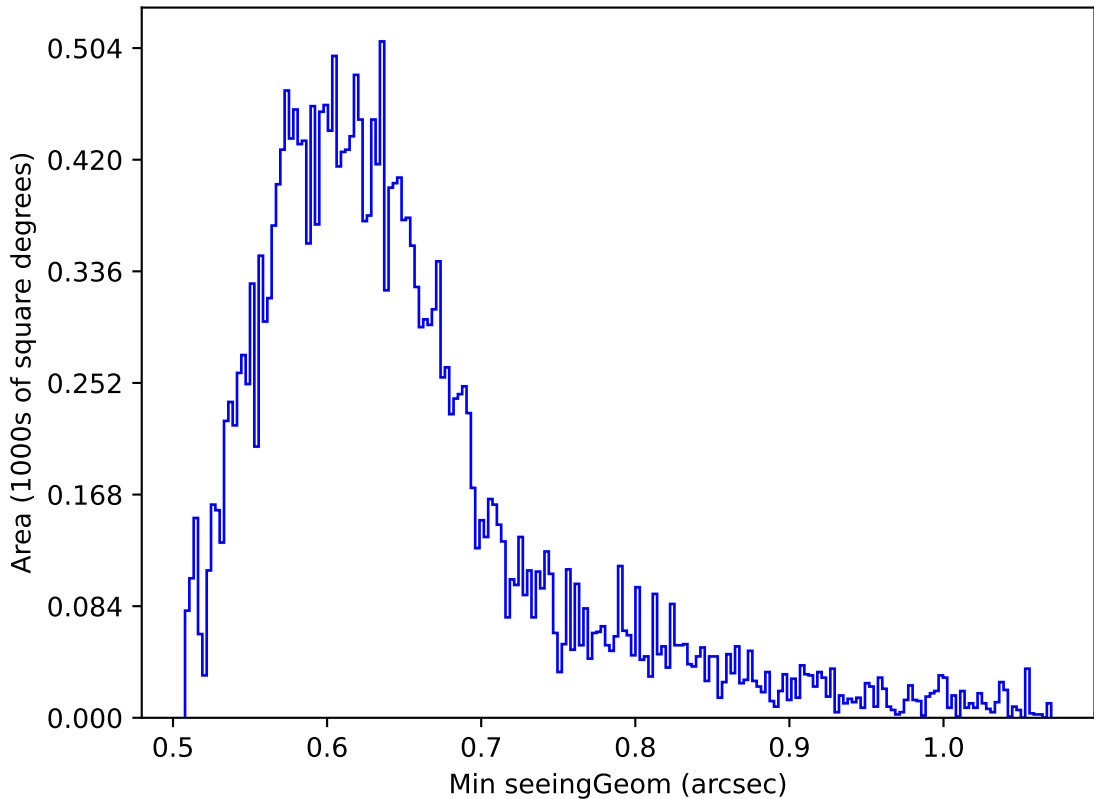
ddf_acor_sf15_lsf40_lsr20_v3.4_10yrs Yr 1 z band: Min seeingGeom
