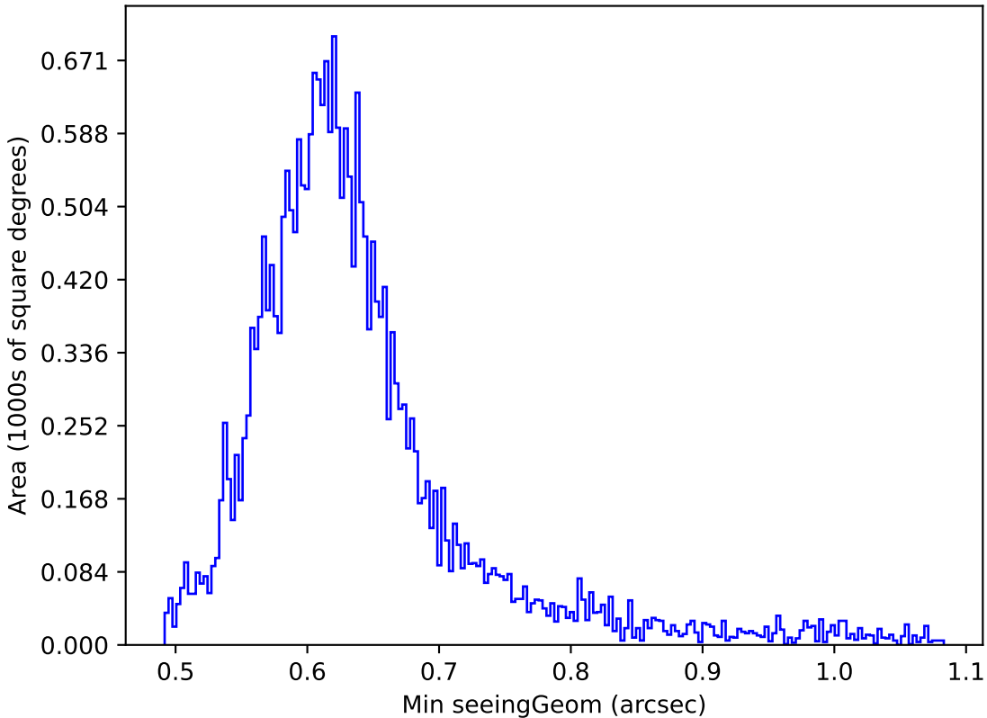
ddf_acor_sf15_lsf40_lsr20_v3.4_10yrs Yr 1 r band: Min seeingGeom
