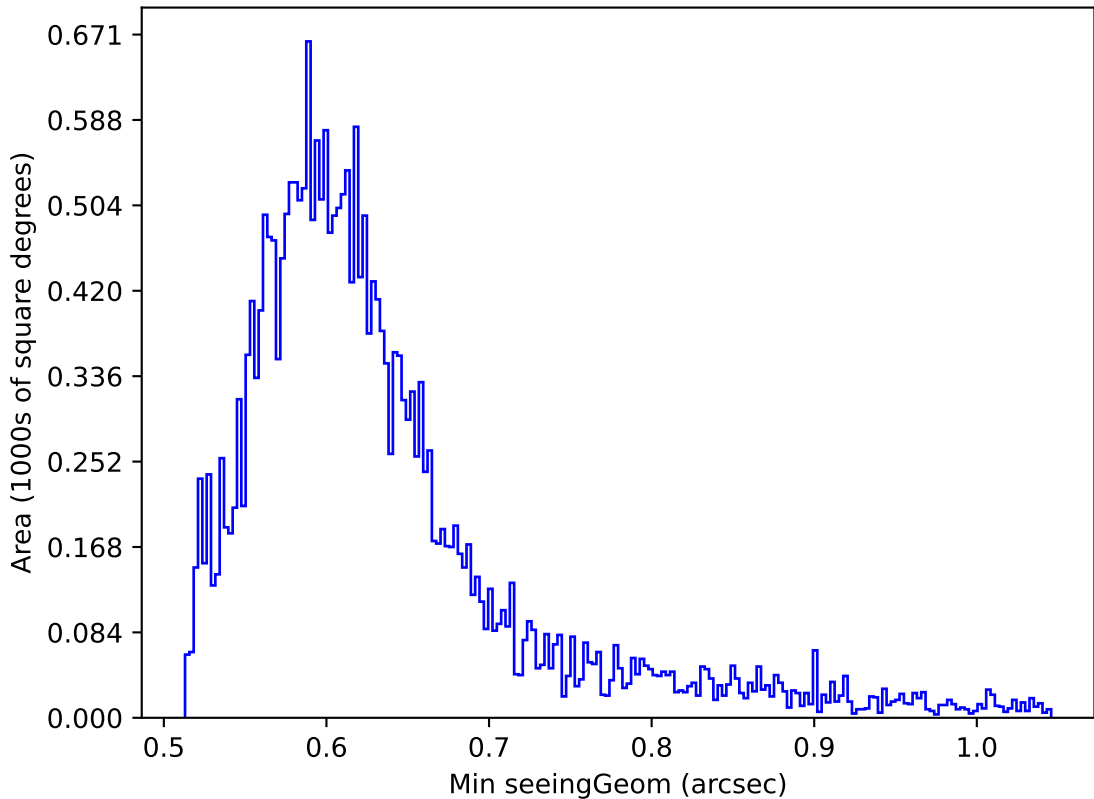
ddf_acor_sf15_lsf40_lsr20_v3.4_10yrs Yr 1 i band: Min seeingGeom
