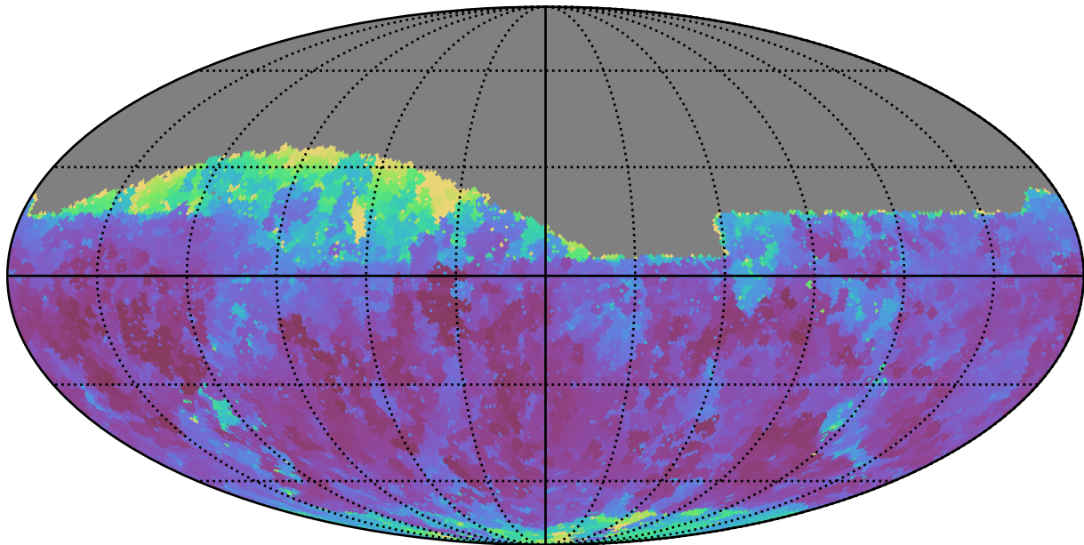
ddf_acor_sf15_lsf40_lsr20_v3.4_10yrs Yr 1 z band: Min seeingEff
