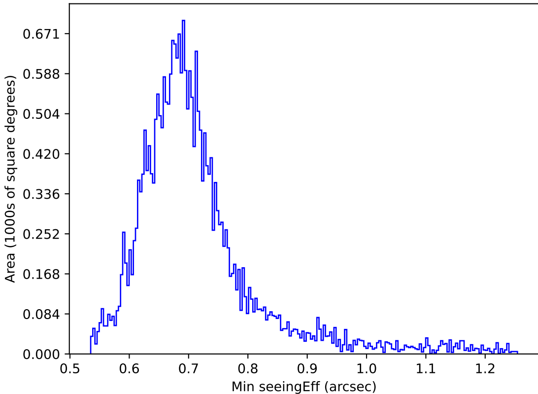
ddf_acor_sf15_lsf40_lsr20_v3.4_10yrs Yr 1 r band: Min seeingEff
