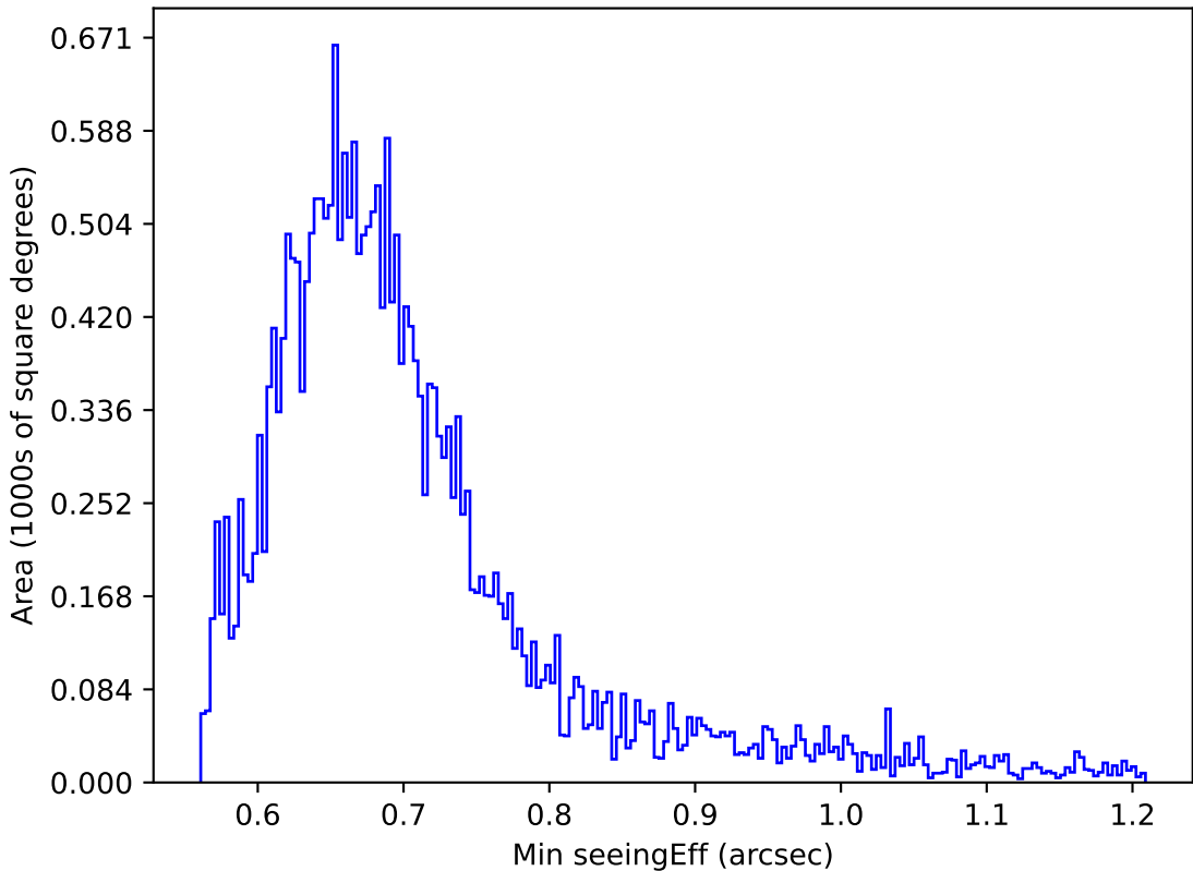
ddf_acor_sf15_lsf40_lsr20_v3.4_10yrs Yr 1 i band: Min seeingEff
