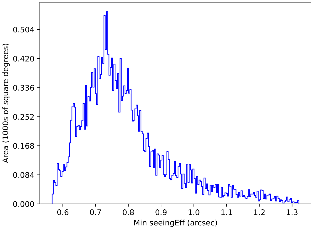
ddf_acor_sf15_lsf40_lsr20_v3.4_10yrs Yr 1 g band: Min seeingEff
