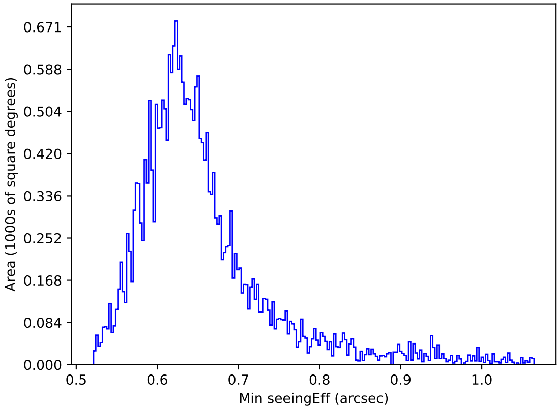
ddf_acor_sf15_lsf40_lsr20_v3.4_10yrs Yr 1 all bands: Min seeingEff
