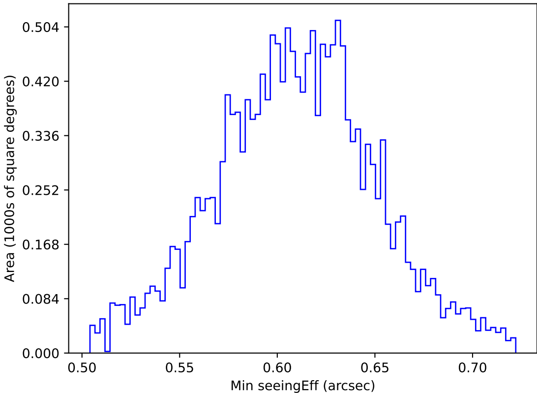
ddf_acor_sf15_lsf40_lsr20_v3.4_10yrs WFD z band: Min seeingEff
