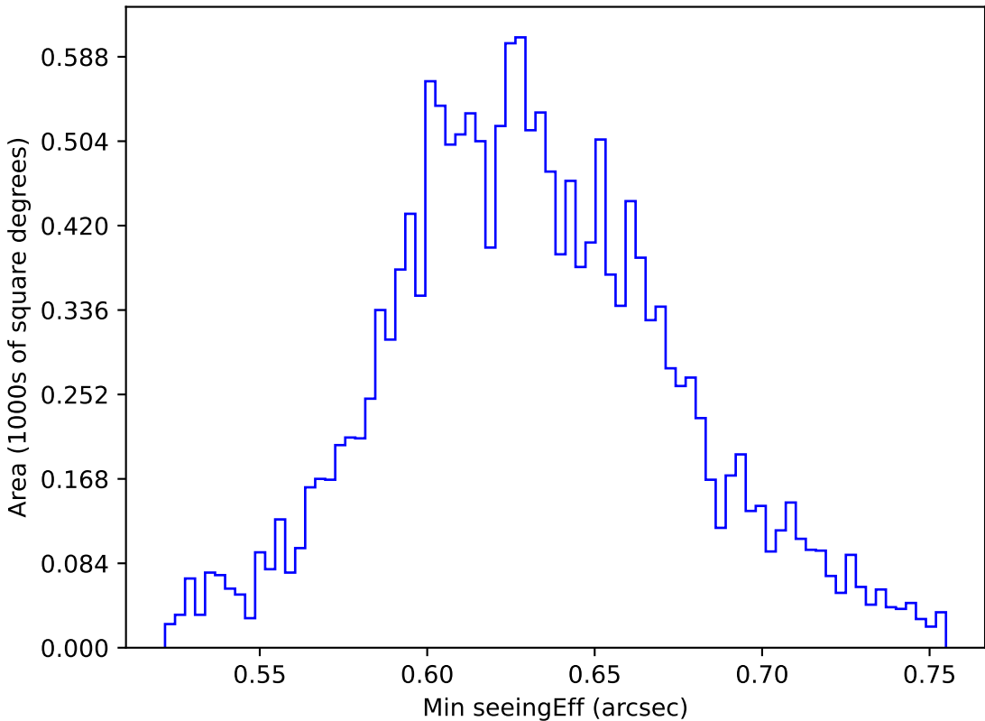
ddf_acor_sf15_lsf40_lsr20_v3.4_10yrs WFD y band: Min seeingEff
