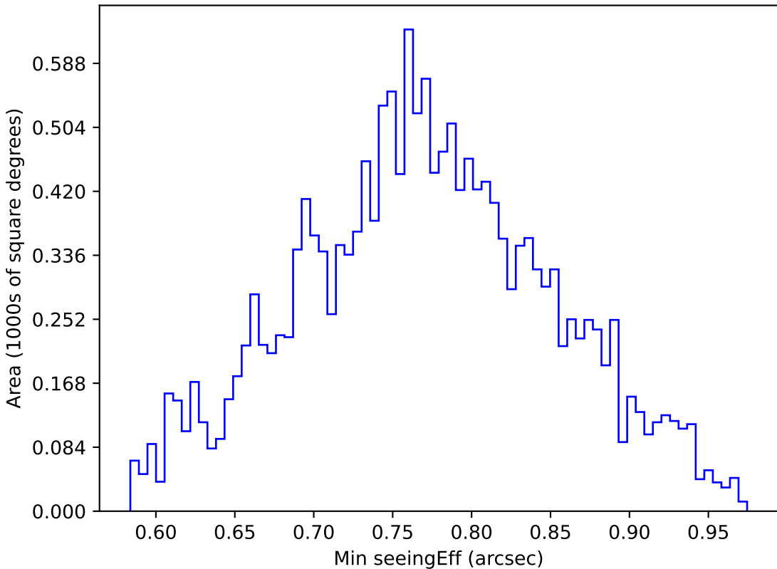
ddf_acor_sf15_lsf40_lsr20_v3.4_10yrs WFD u band: Min seeingEff
