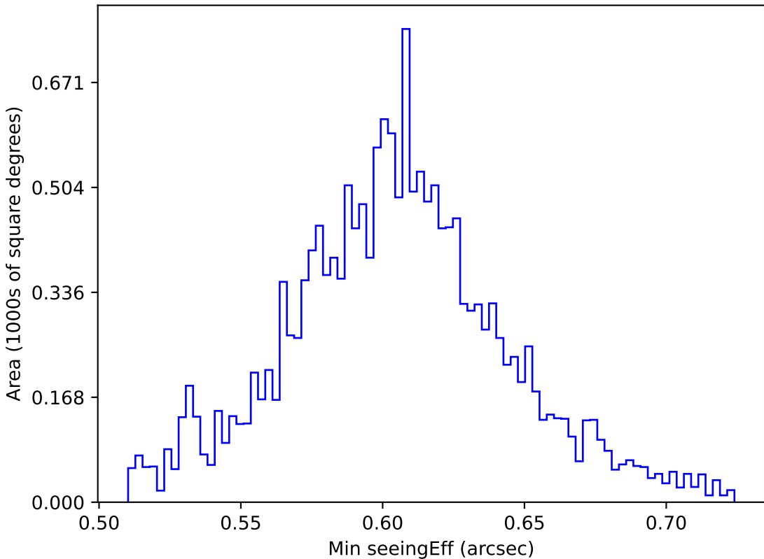
ddf_acor_sf15_ls40_lsr20_v3.4_10yrs WFD i band: Min seeingEff
