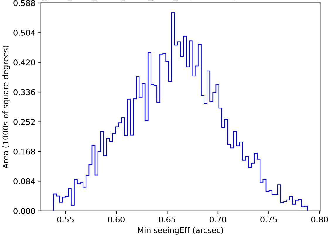
ddf_acor_sf15_lsf40_lsr20_v3.4_10yrs WFD g band: Min seeingEff
