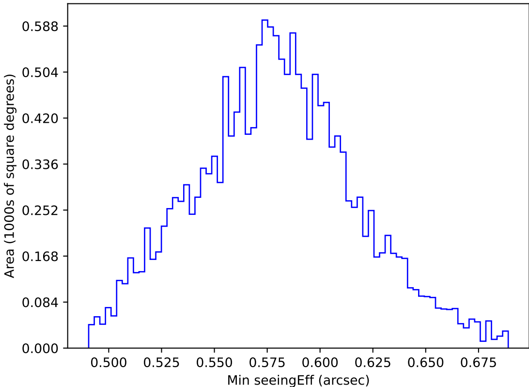
ddf_acor_sf15_lsf40_lsr20_v3.4_10yrs WFD all bands: Min seeingEff
