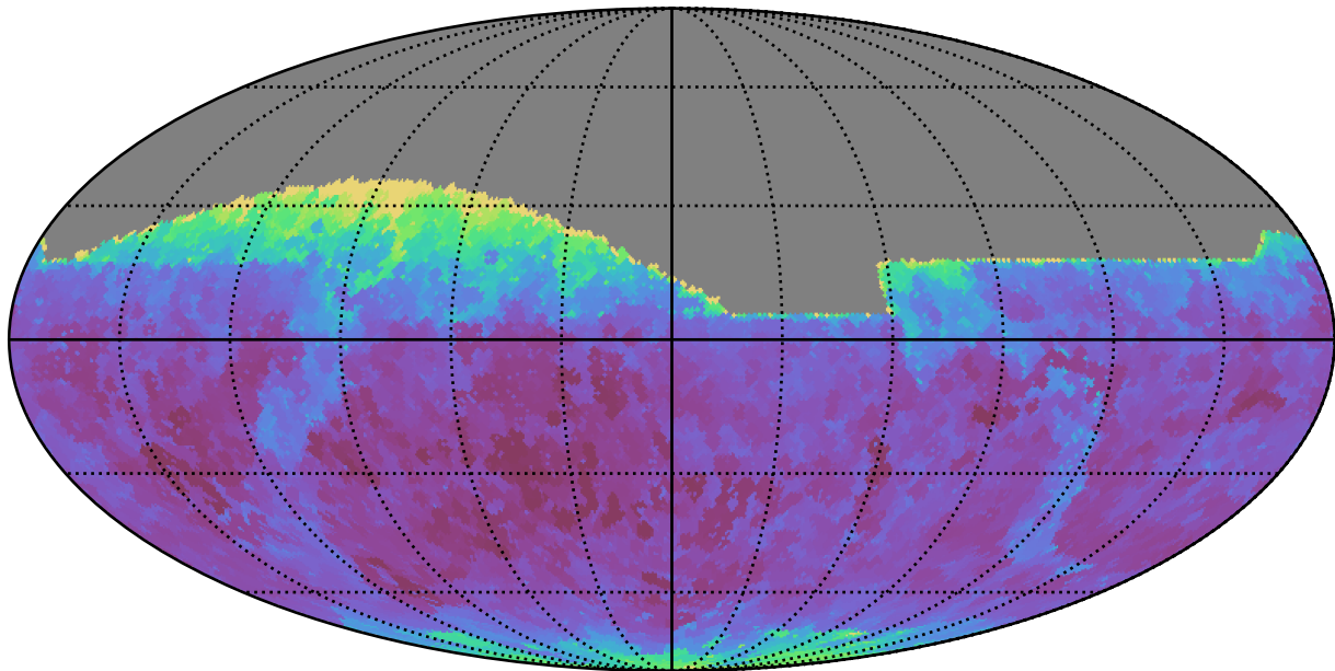
ddf_acor_sf15_lsf40_lsr20_v3.4_10yrs All sky z band: Min seeingEff
