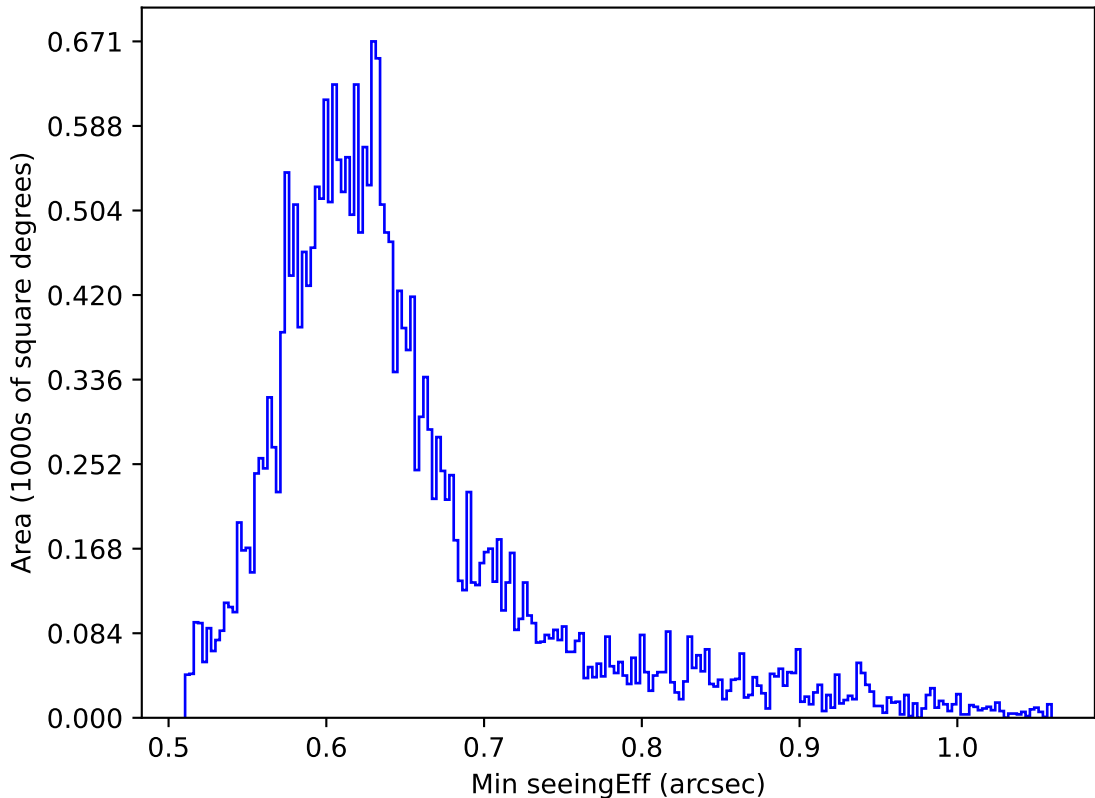
ddf_acor_sf15_lsf40_lsr20_v3.4_10yrs All sky z band: Min seeingEff
