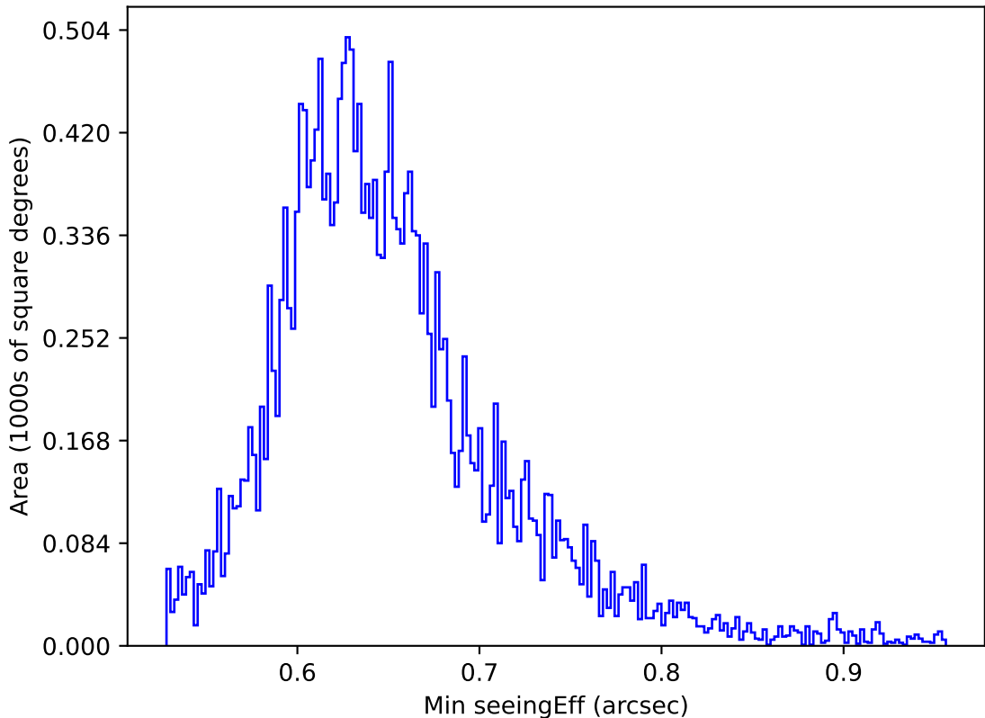
ddf_acor_sf15_lsf40_lsr20_v3.4_10yrs All sky y band: Min seeingEff
