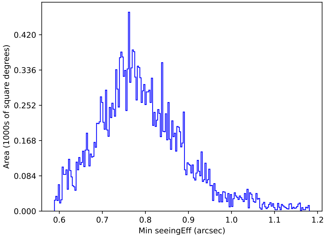
ddf_acor_sf15_lsf40_lsr20_v3.4_10yrs All sky u band: Min seeingEff
