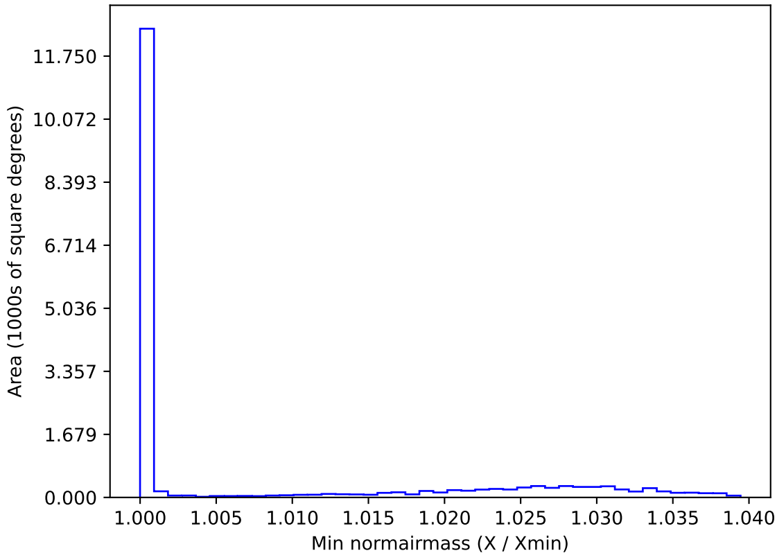
ddf_acor_sf15_lsf40_lsr20_v3.4_10yrs WFD y band: Min normairmass
