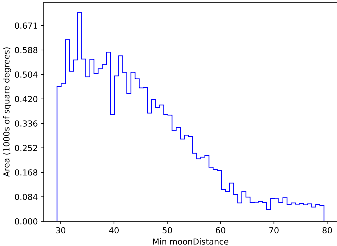
ddf_acor_sf15_lsf40_lsr20_v3.4_10yrs WFD g band: Min moonDistance
