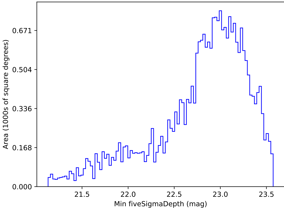
ddf_acor_sf15_lsf40_lsr20_v3.4_10yrs Yr 1 i band: Min fiveSigmaDepth
