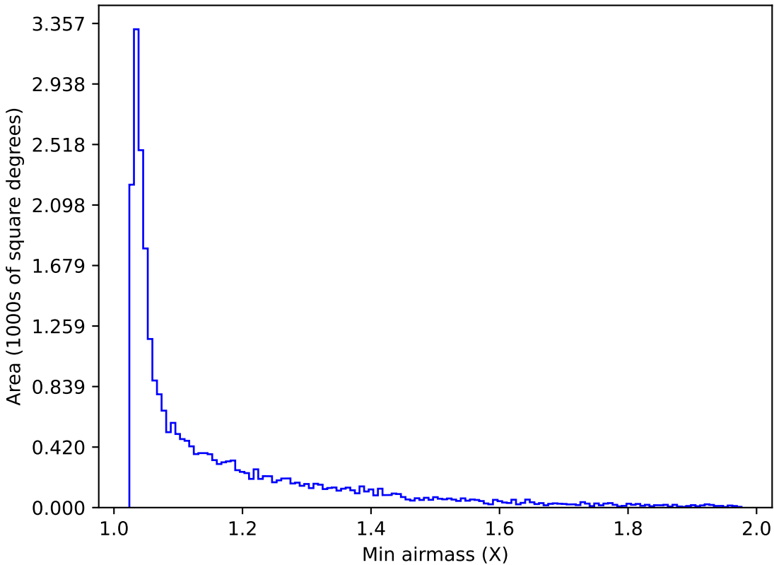
ddf_acor_sf15_lsf40_lsr20_v3.4_10yrs Yr 1 i band: Min airmass
