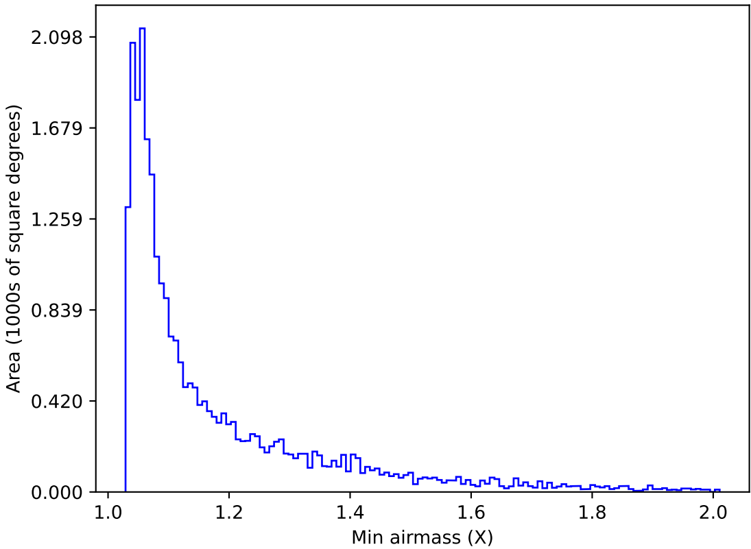
ddf_acor_sf15_lsf40_lsr20_v3.4_10yrs Yr 1 g band: Min airmass
