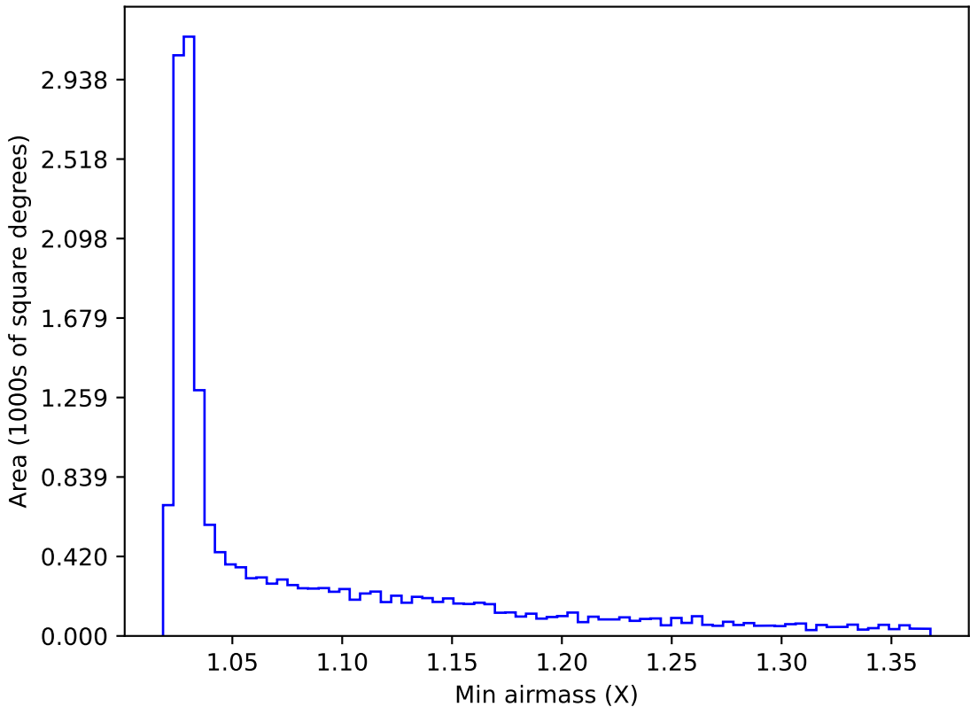
ddf_acor_sf15_lsf40_lsr20_v3.4_10yrs WFD z band: Min airmass
