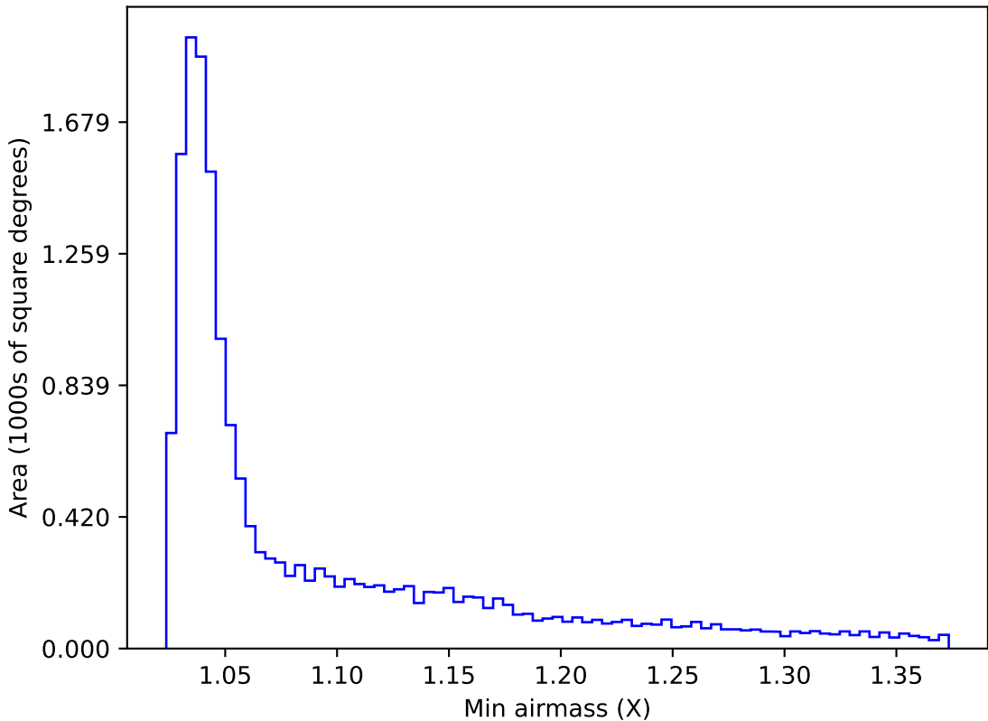
ddf_acor_sf15_lsf40_lsr20_v3.4_10yrs WFD u band: Min airmass
