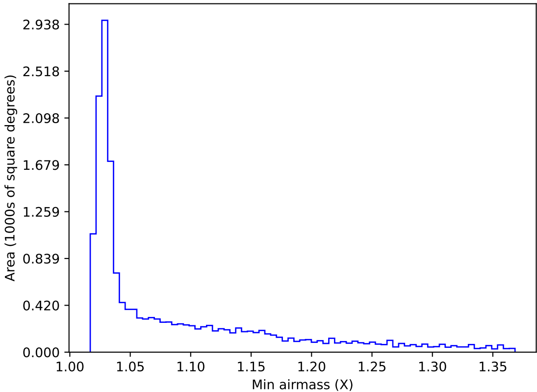
ddf_acor_sf15_lsf40_lsr20_v3.4_10yrs WFD r band: Min airmass
