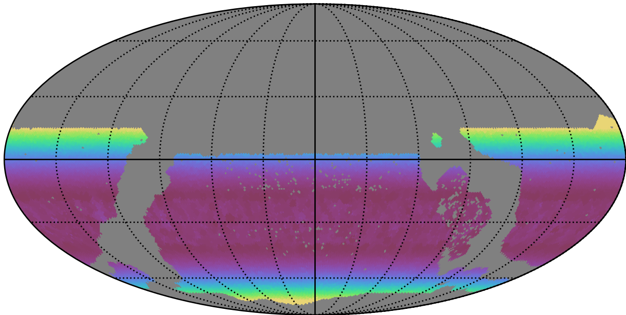
ddf_acor_sf15_lsf40_lsr20_v3.4_10yrs WFD g band: Min airmass
