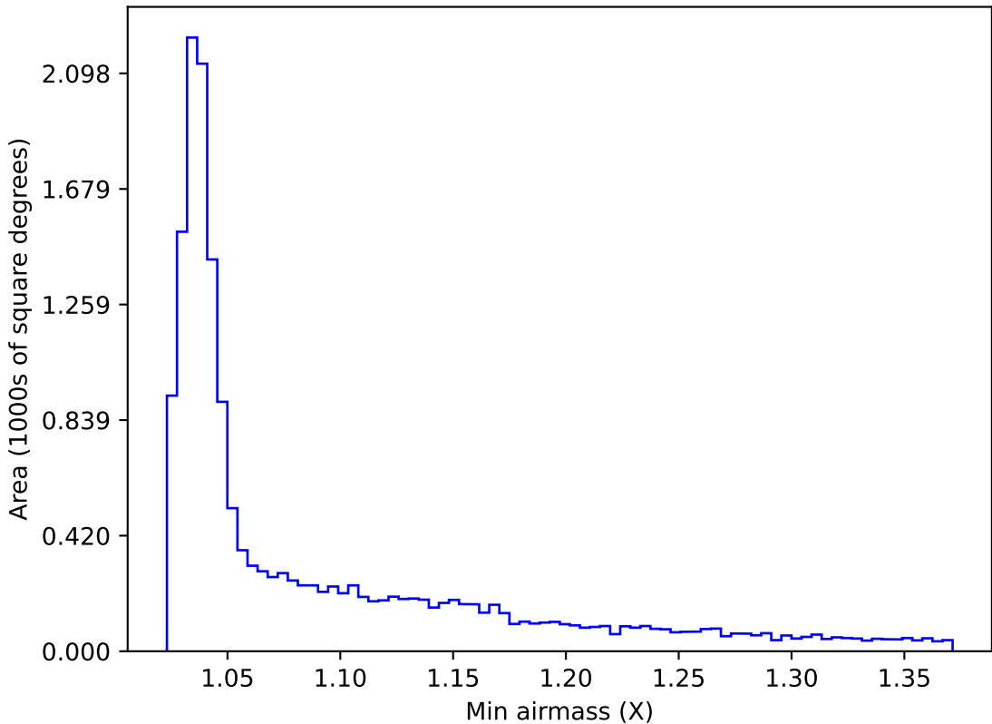
ddf_acor_sf15_lsf40_lsr20_v3.4_10yrs WFD g band: Min airmass
