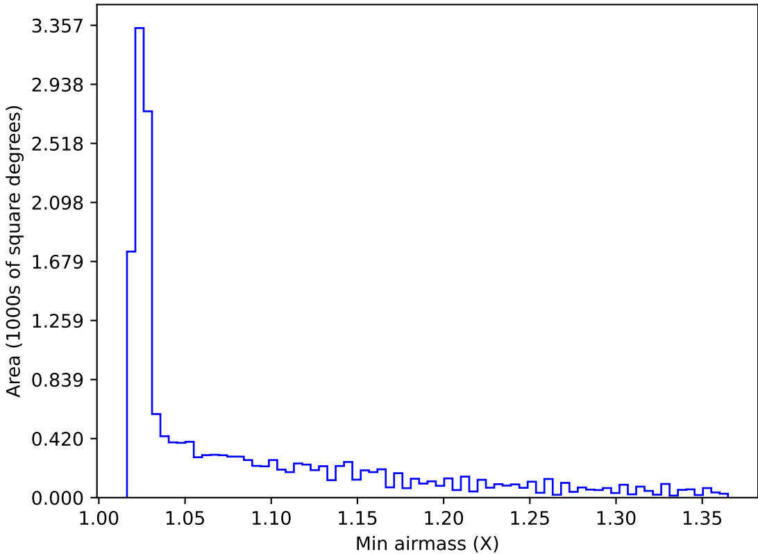
ddf_acor_sf15_lsf40_lsr20_v3.4_10yrs WFD all bands: Min airmass
