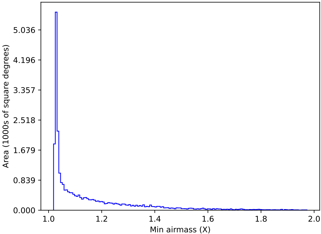
ddf_acor_sf15_lsf40_lsr20_v3.4_10yrs All sky z band: Min airmass
