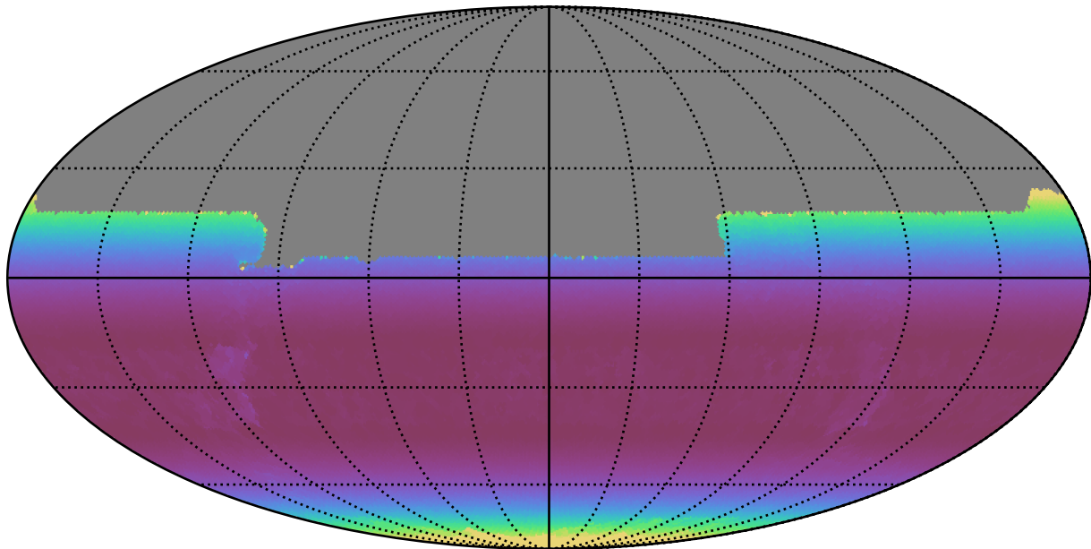
ddf_acor_sf15_lsf40_lsr20_v3.4_10yrs All sky y band: Min airmass
