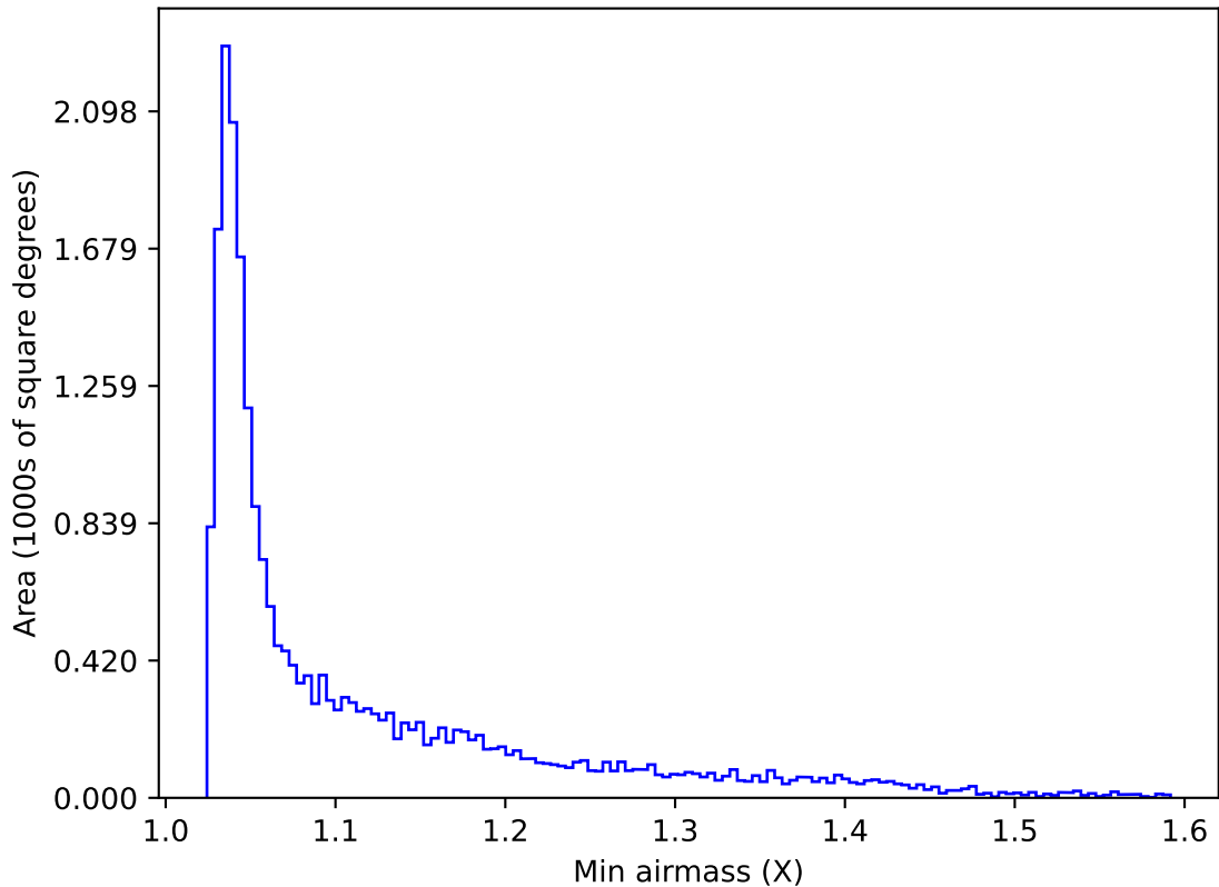
ddf_acor_sf15_lsf40_lsr20_v3.4_10yrs All sky u band: Min airmass
