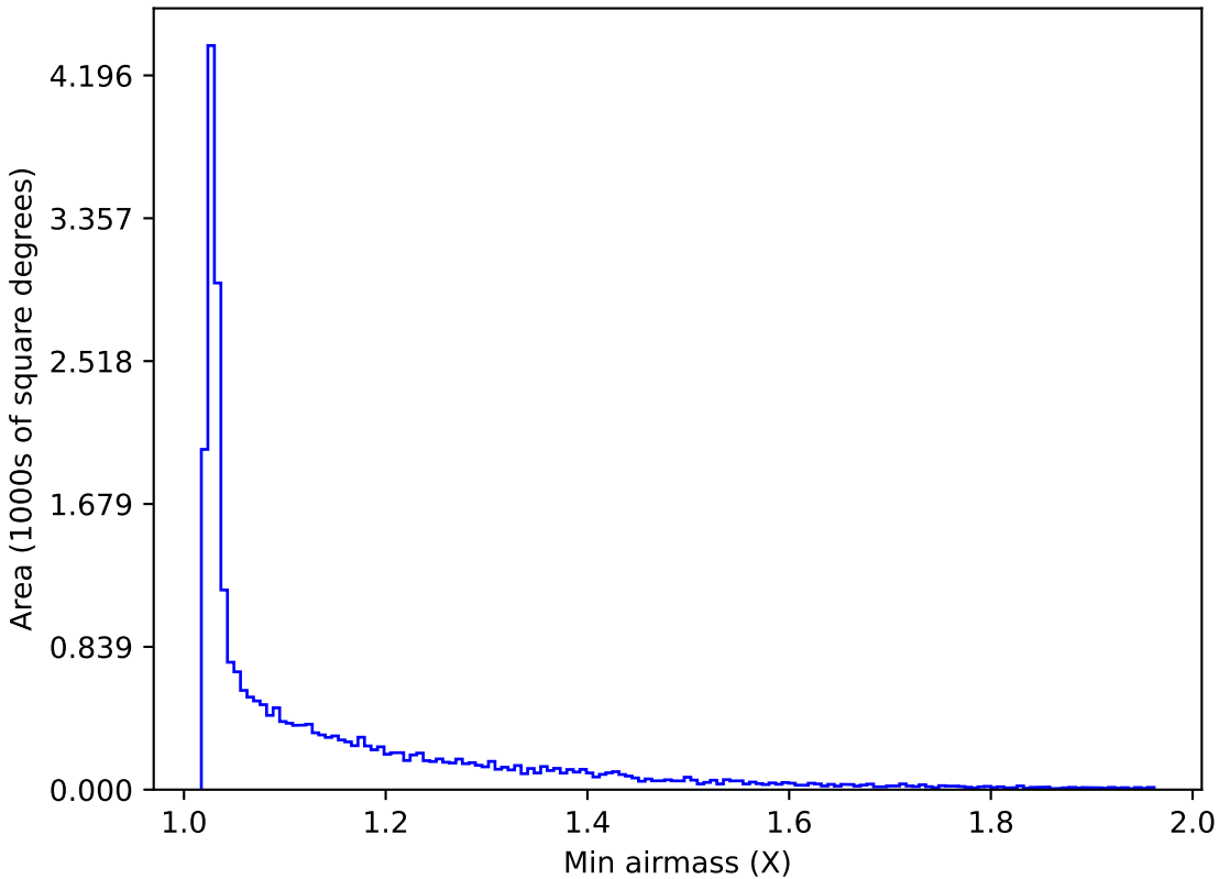
ddf_acor_sf15_lsf40_lsr20_v3.4_10yrs All sky r band: Min airmass
