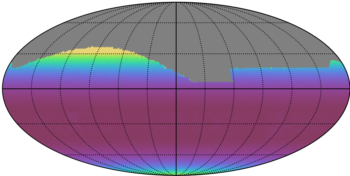
ddf_acor_sf15_lsf40_lsr20_v3.4_10yrs All sky i band: Min airmass
