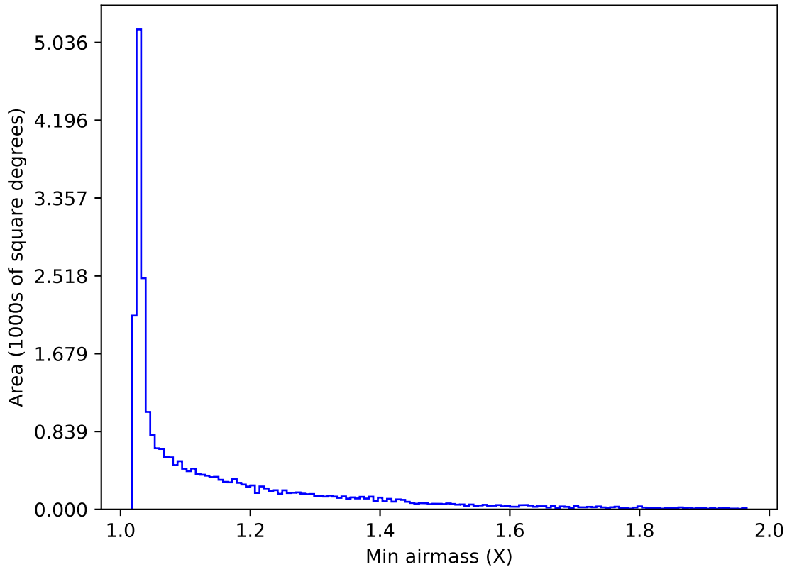
ddf_acor_sf15_lsf40_lsr20_v3.4_10yrs All sky i band: Min airmass
