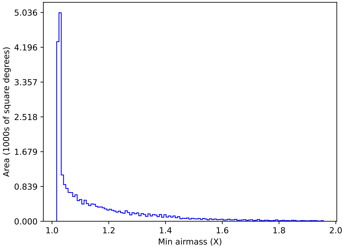
ddf_acor_sf15_lsf40_lsr20_v3.4_10yrs All sky all bands: Min airmass
