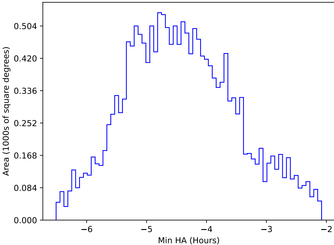
ddf_acor_sf15_lsf40_lsr20_v3.4_10yrs WFD z band: Min HA
