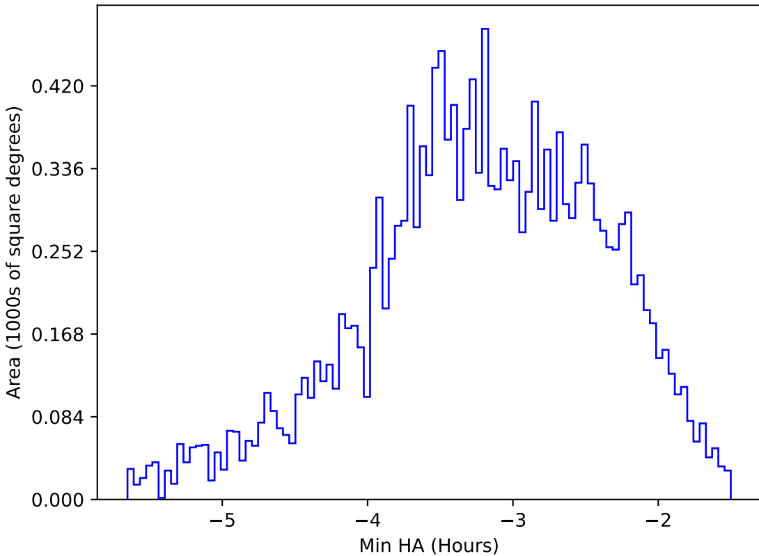
ddf_acor_sf15_lsf40_lsr20_v3.4_10yrs WFD u band: Min HA
