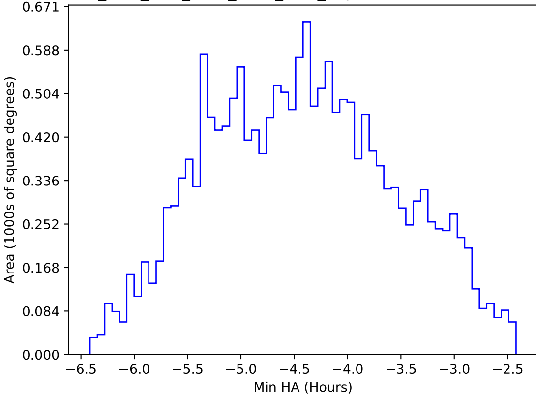
ddf_acor_sf15_lsf40_lsr20_v3.4_10yrs WFD r band: Min HA
