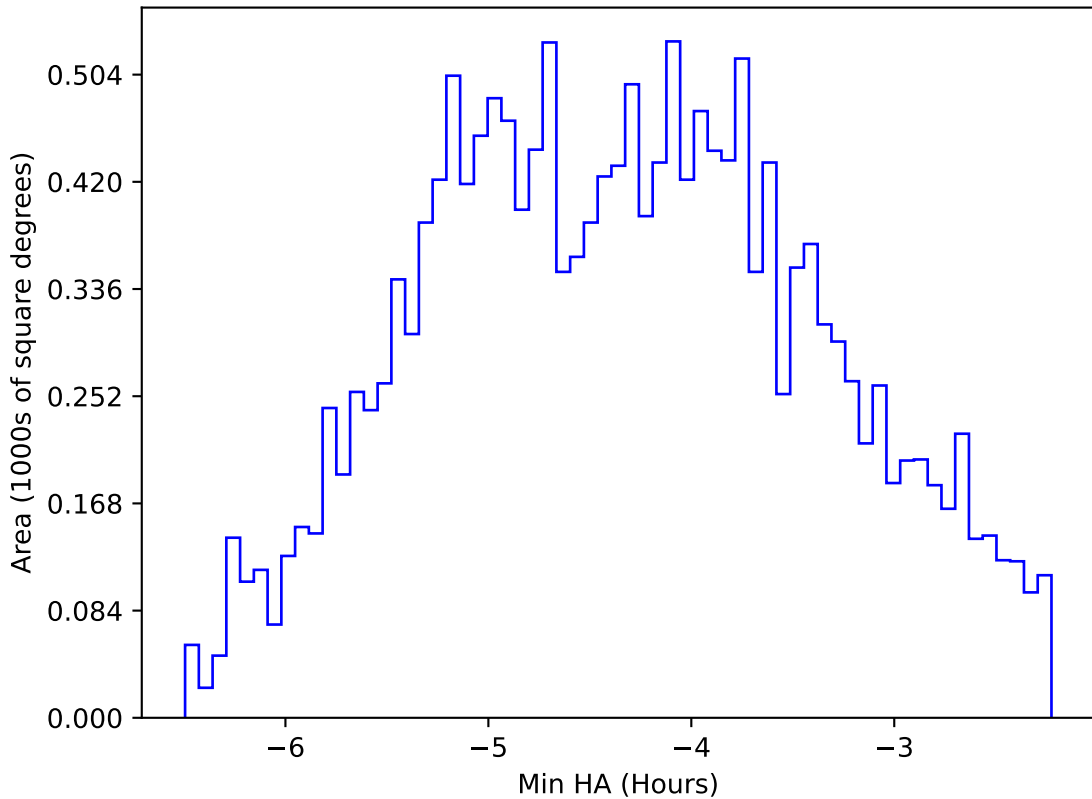
ddf_acor_sf15_lsf40_lsr20_v3.4_10yrs WFD i band: Min HA
