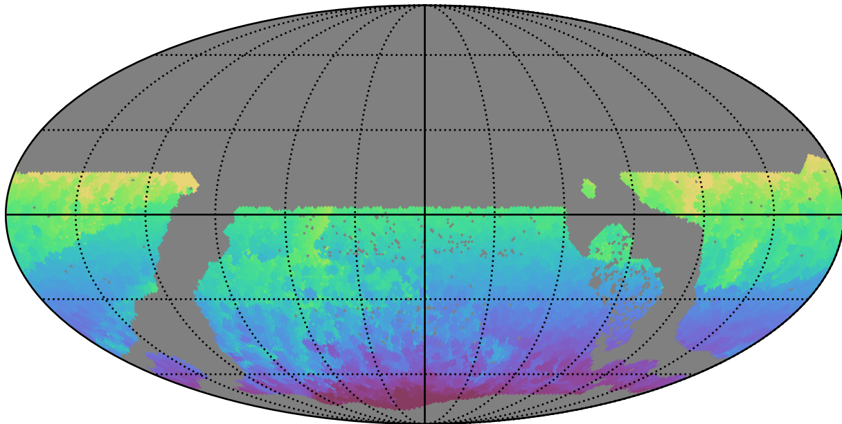
ddf_acor_sf15_lsf40_lsr20_v3.4_10yrs WFD all bands: Min HA
