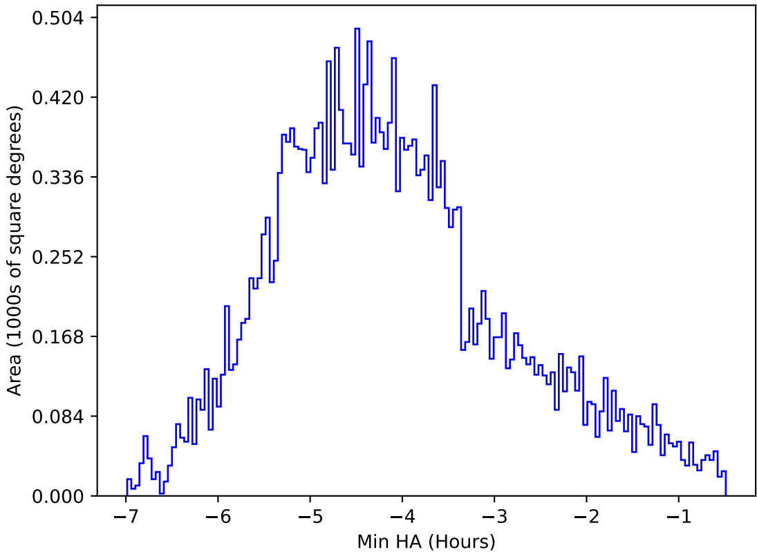
ddf_acor_sf15_lsf40_lsr20_v3.4_10yrs All sky z band: Min HA
