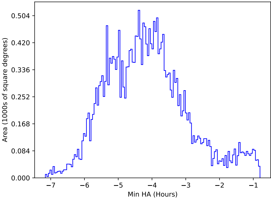
ddf_acor_sf15_ls40_lsr20_v3.4_10yrs All sky r band: Min HA
