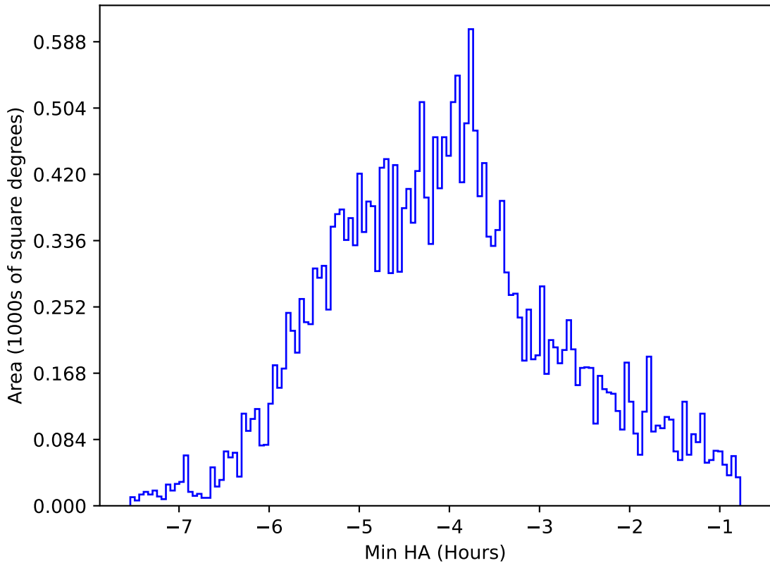
ddf_acor_sf15_lsf40_lsr20_v3.4_10yrs All sky i band: Min HA
