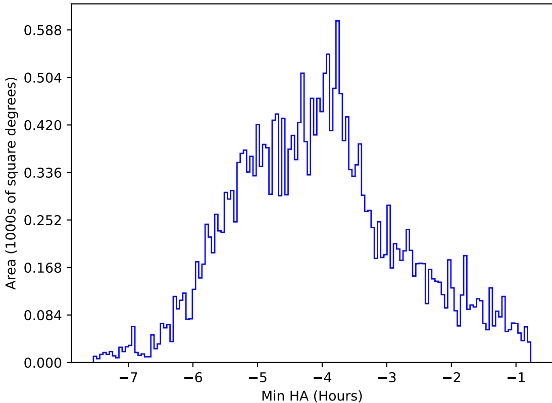
ddf_acor_sf15_ls40_lsr20_v3.4_10yrs All sky i band: Min HA
