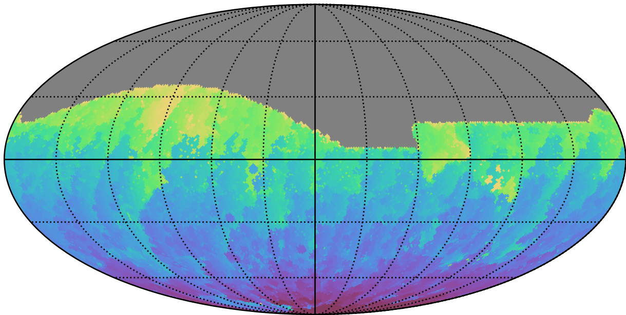
ddf_acor_sf15_lsf40_lsr20_v3.4_10yrs All sky g band: Min HA
