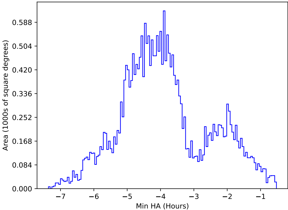
ddf_acor_sf15_lsf40_lsr20_v3.4_10yrs All sky g band: Min HA
